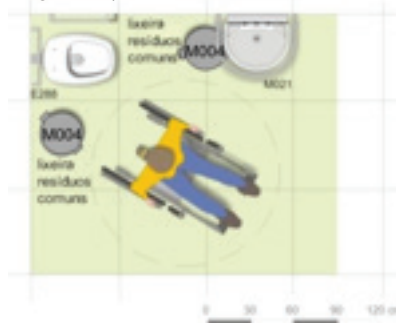
Figura 80: Layout.
