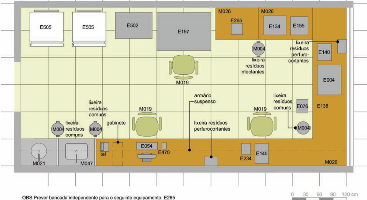
Figura 43: Layout.
