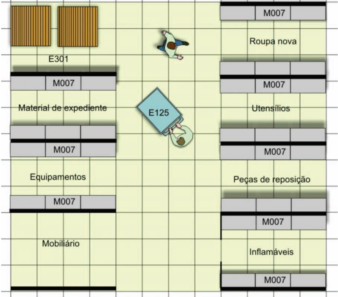
Figura 69: Layout.
