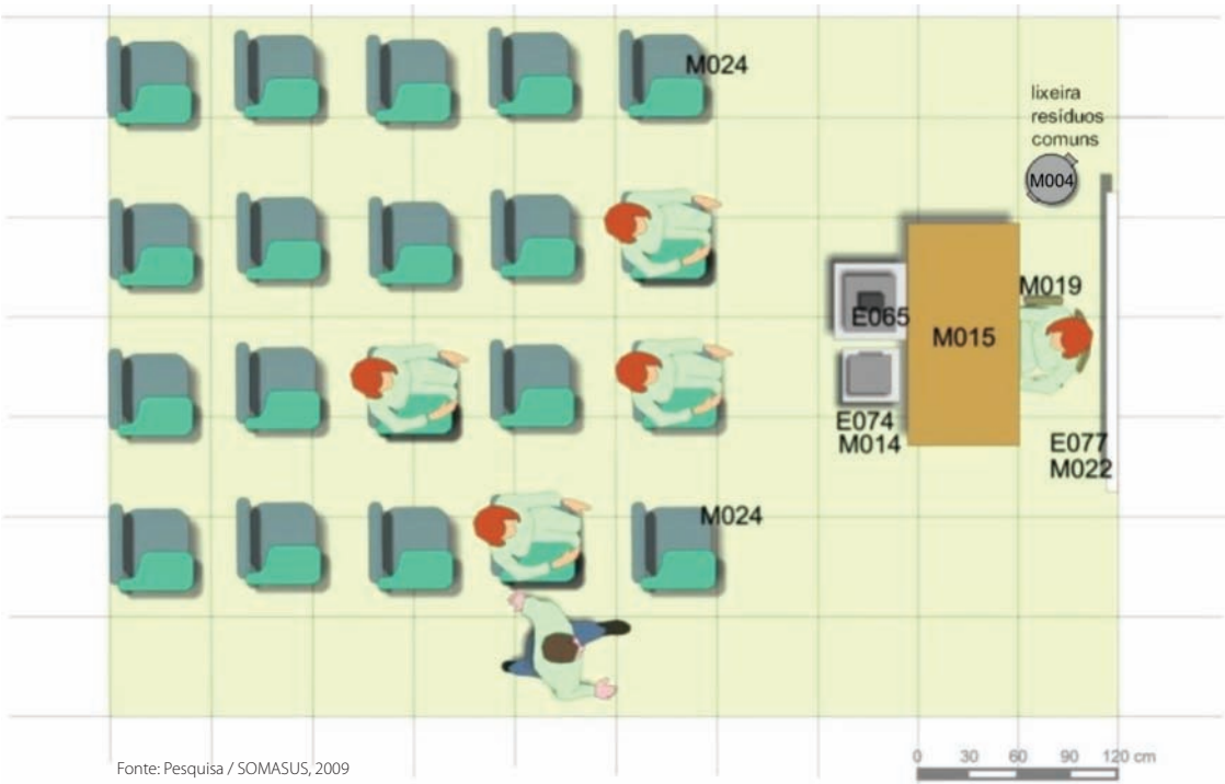
Figura 63: Layout.
