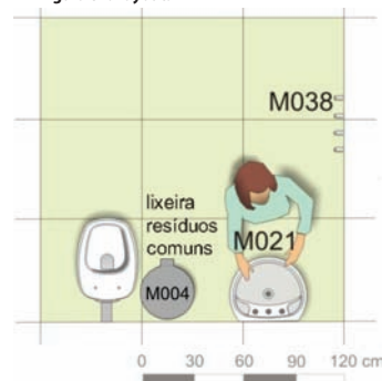
Figura 81: Layout.
