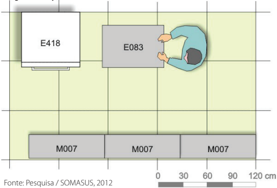
Figura 72: Layout.
