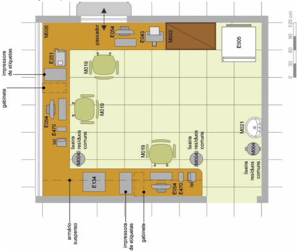
Figura 41: Layout.
