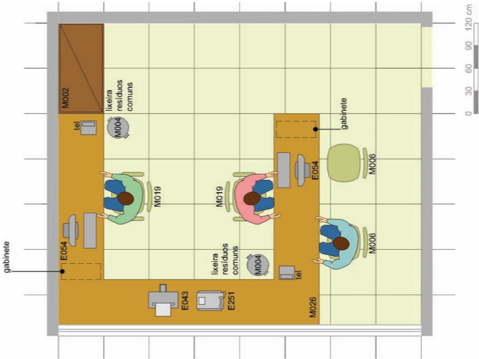
Figura 61: Layout.
