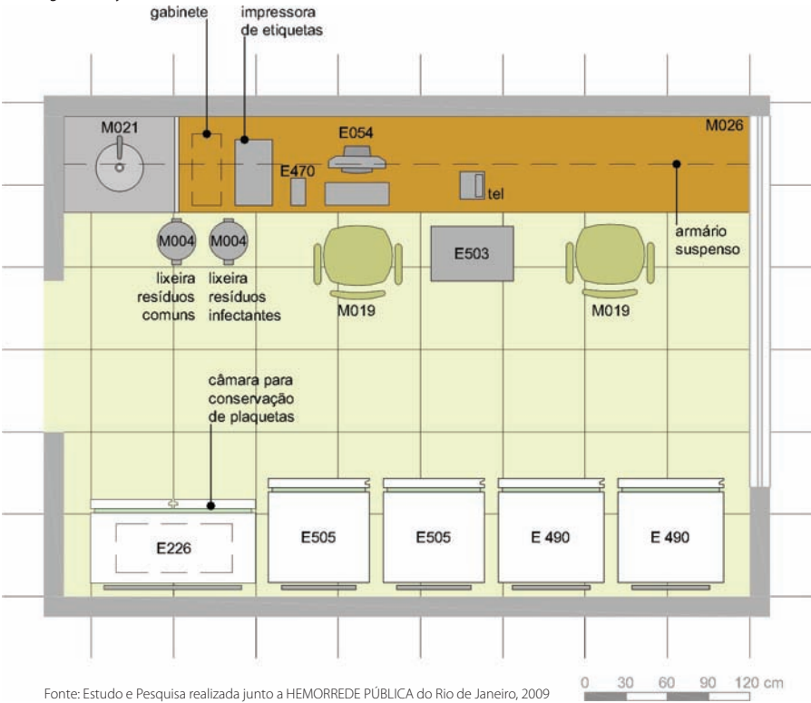
Figura 53: Layout.
