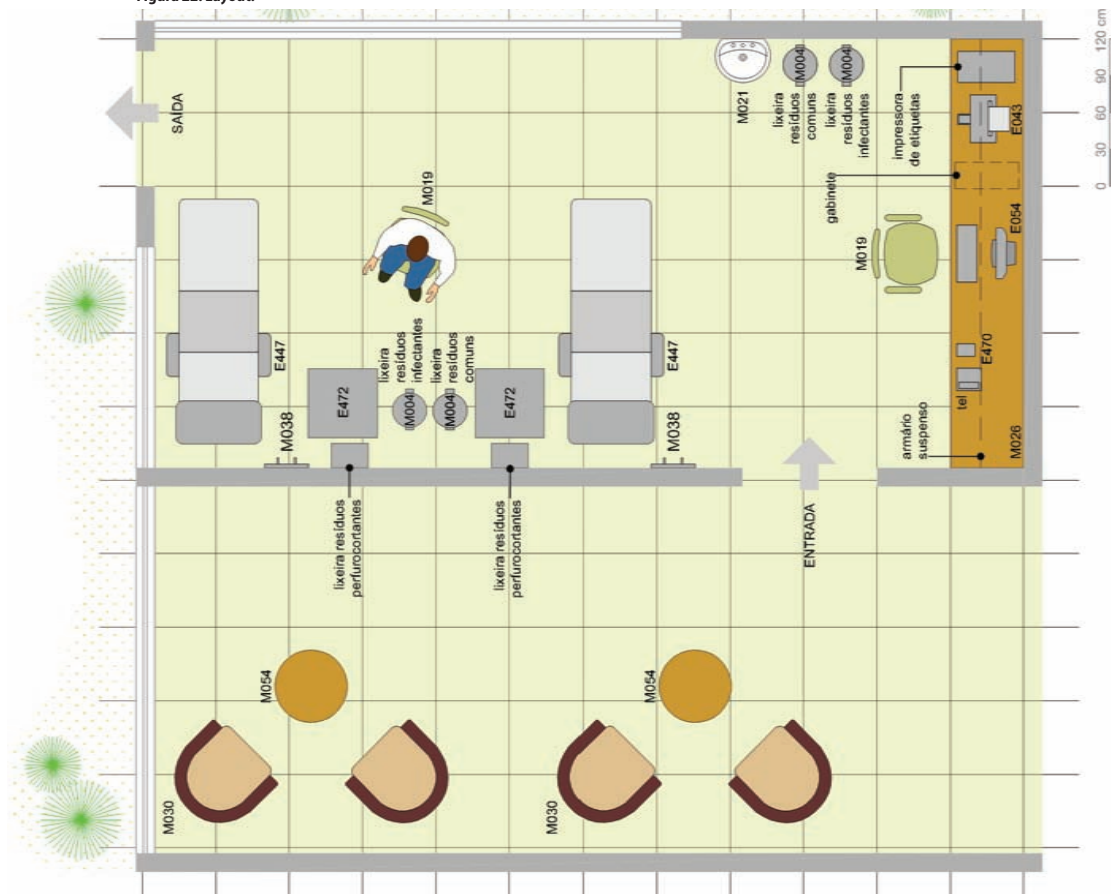
Figura 22: Layout.
