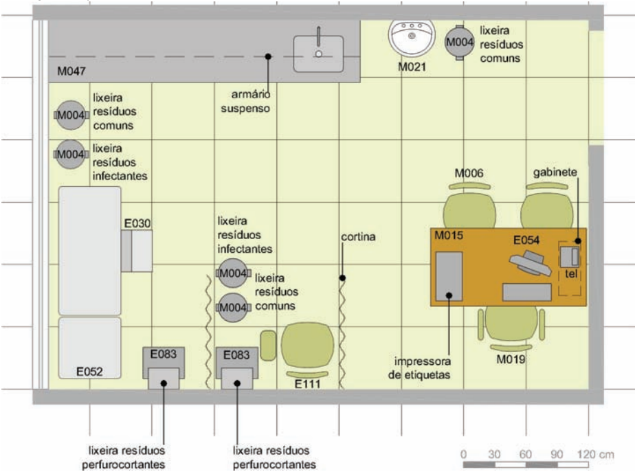
Figura 32: Layout.
