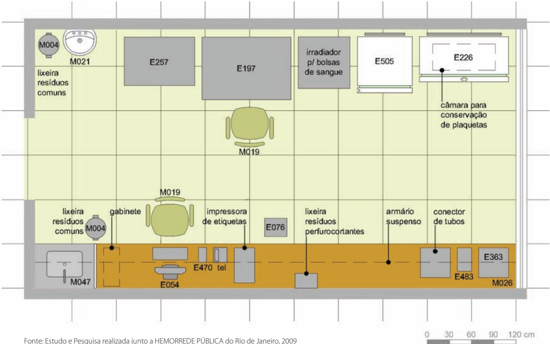
Figura 54: Layout.
