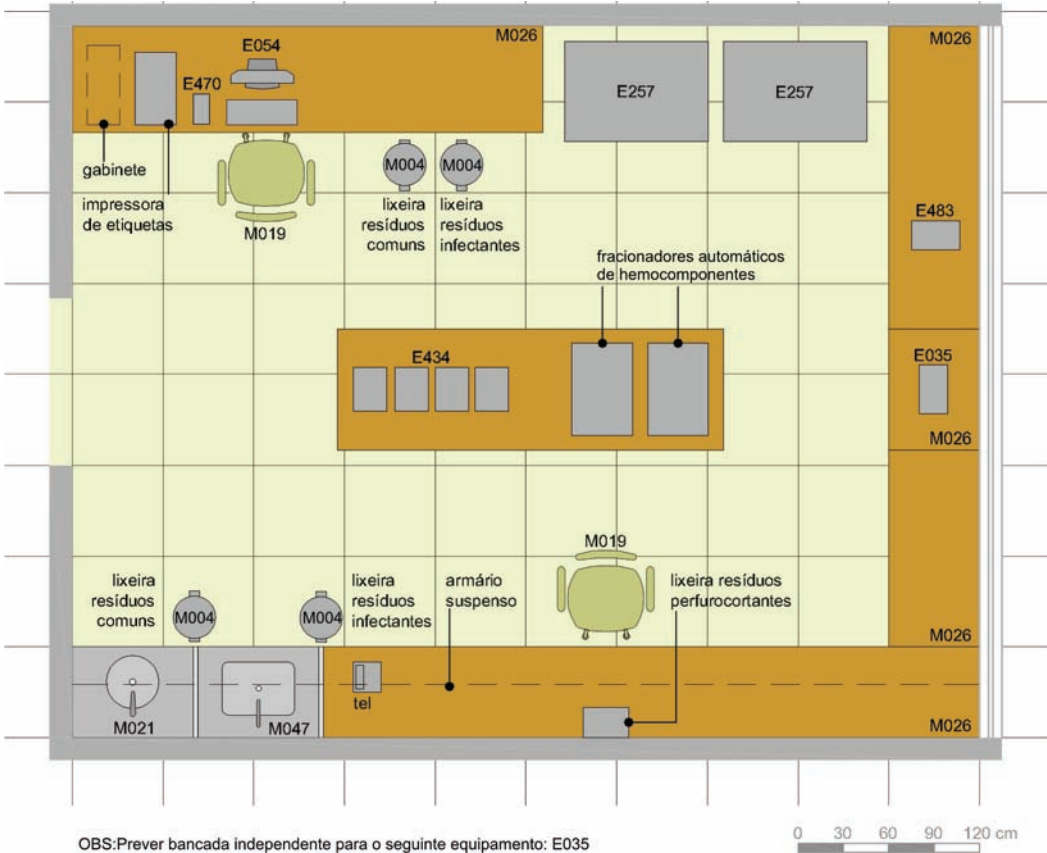
Figura 55: Layout.
